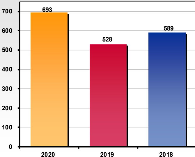
Cooling Degree Days--YTD April - July
